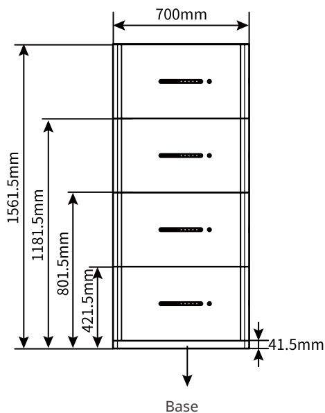
Battery group dimensions (ground installation)
