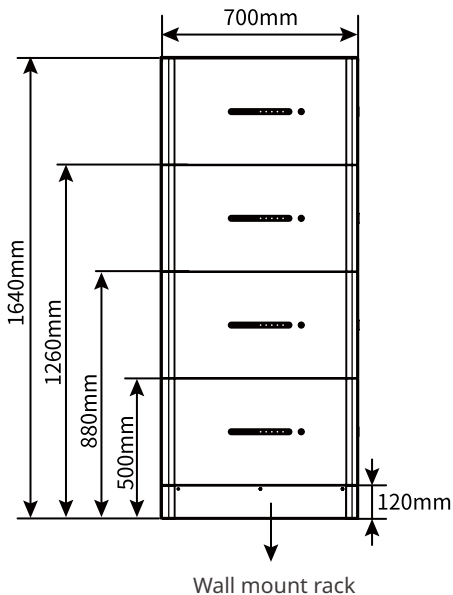
Battery group dimensions (wall-mount installation)
